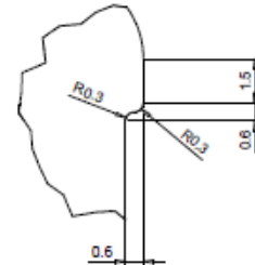
TYPICAL PANEL TRANSITION ( 10 : 1 )
