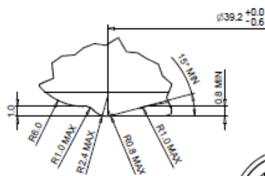
STACKING RING ( 5 : 1 ) CONFORMS TO F.D. 114
