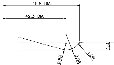
STACKING RING DETAIL SCALE 10:1
